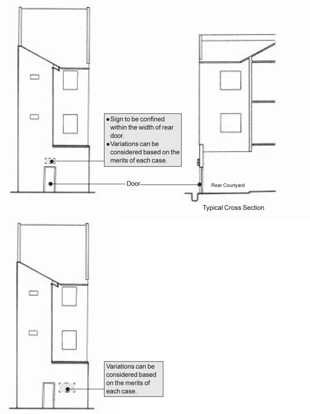
Figure 9 : Rear Wall
