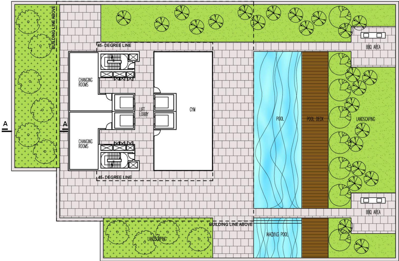
5TH STOREY LANDSCAPE PLAN (To Indicate Scale)
