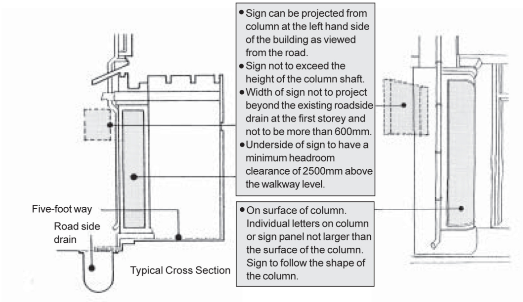
Figure 4 : First Storey Column
