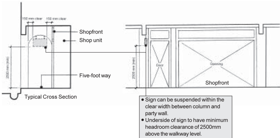
Figure 4 : First Storey Column
