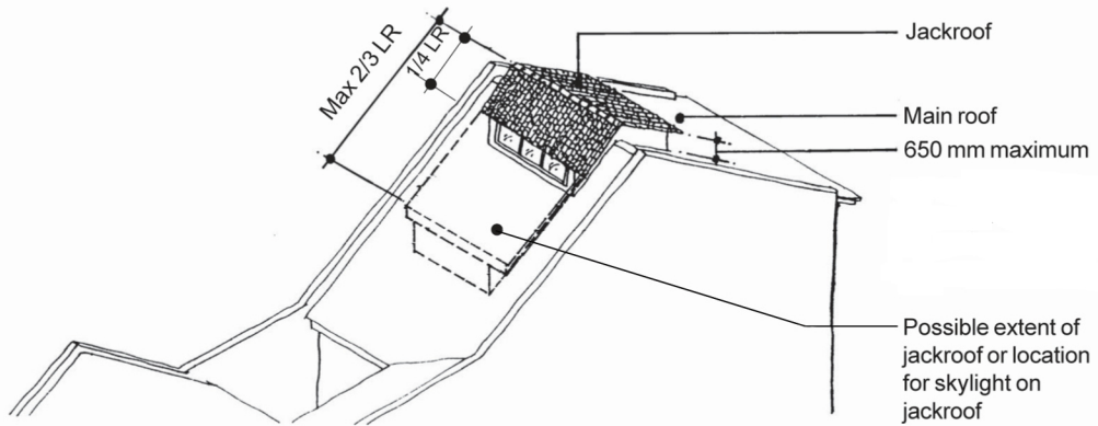
ISOMETRIC VIEW
