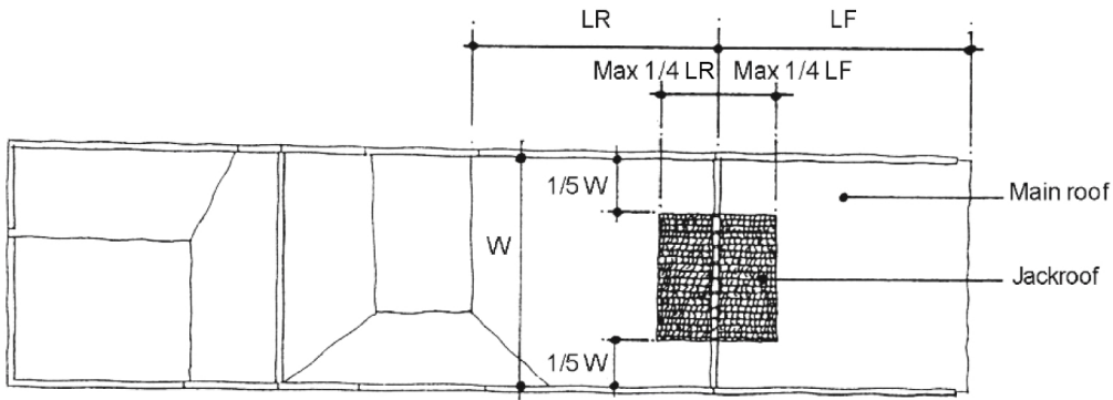
ROOF PLAN
