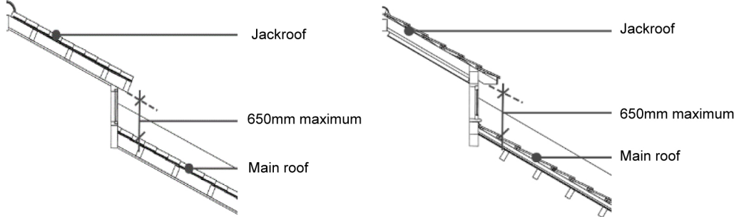
Jackroof with v-profile roof tiles
