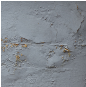
Application of impervious surface finishes such as cement-based render and film-forming paint systems can worsen the situation by trapping moisture within the wall. In the image above, trapped moisture under the paint resulted in a bubbling appearance, peeling, and cracks on the surface of the wall.
