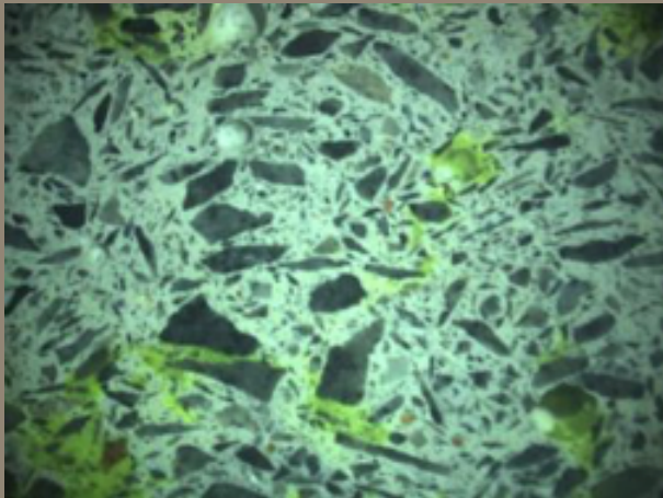
A polished section of Shanghai plaster made up of white Portland cement and crushed granite chips.
